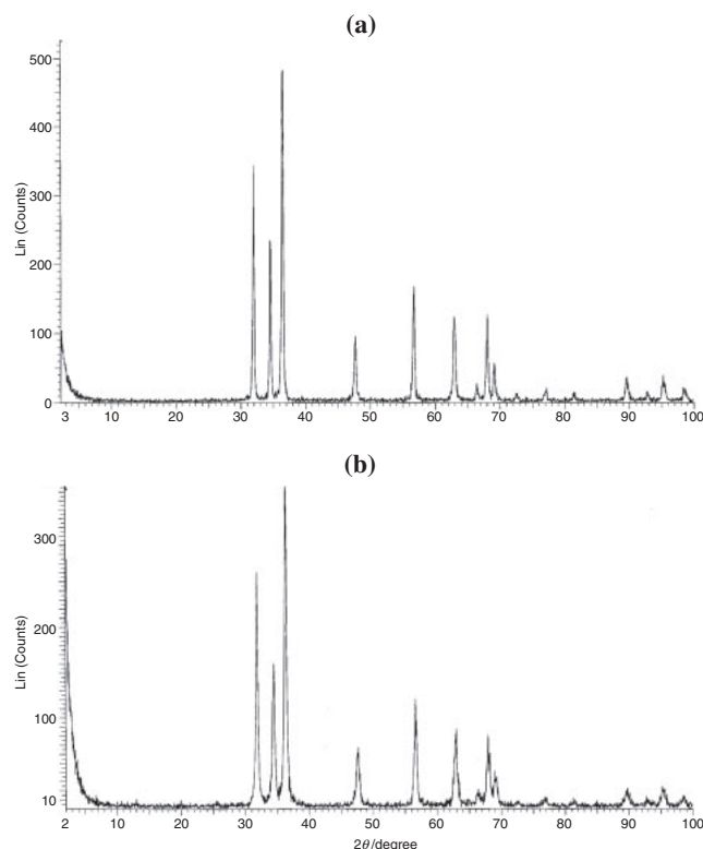
Figure 1. The XRD patterns of ZnO; (a) before reaction, (b) after reaction.
